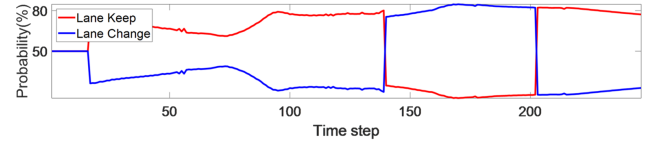
(c) Predicted Lane change probability over time
