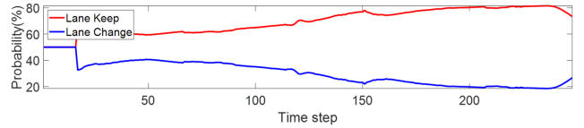
(b) Predicted Lane change probability over time
